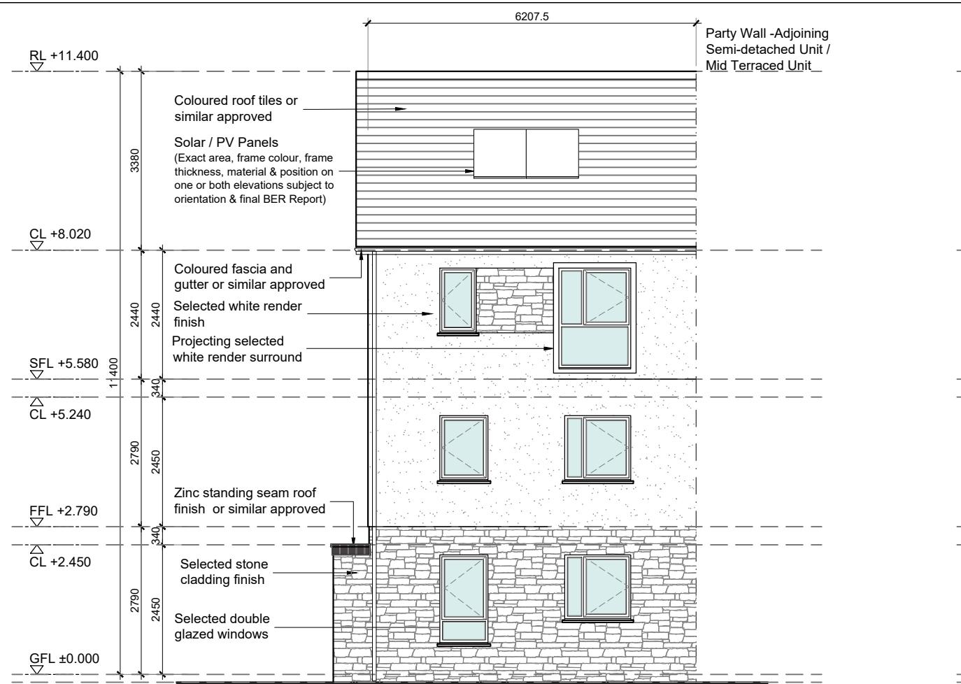
01 Front Elevation 1:100 @ A3
