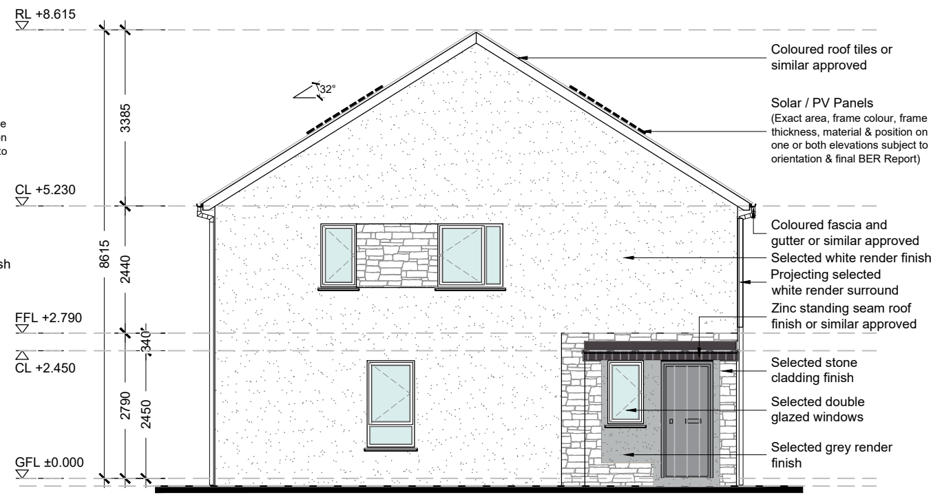
04 Side Elevation - Unit 125 only 1:100 @ A3
