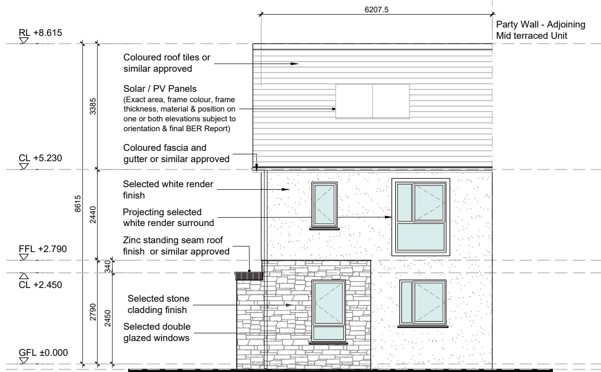
01 Front Elevation 1:100 @ A3
