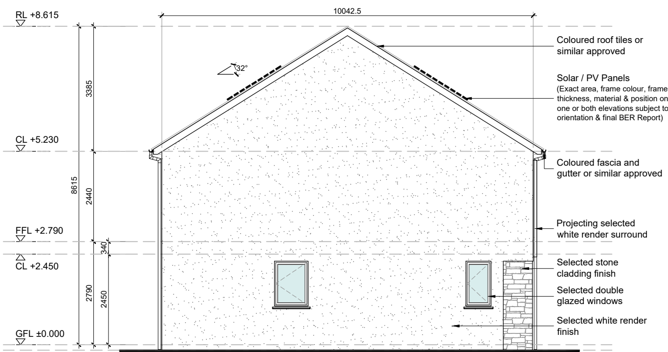
03 Side Elevation 1:100 @ A3
