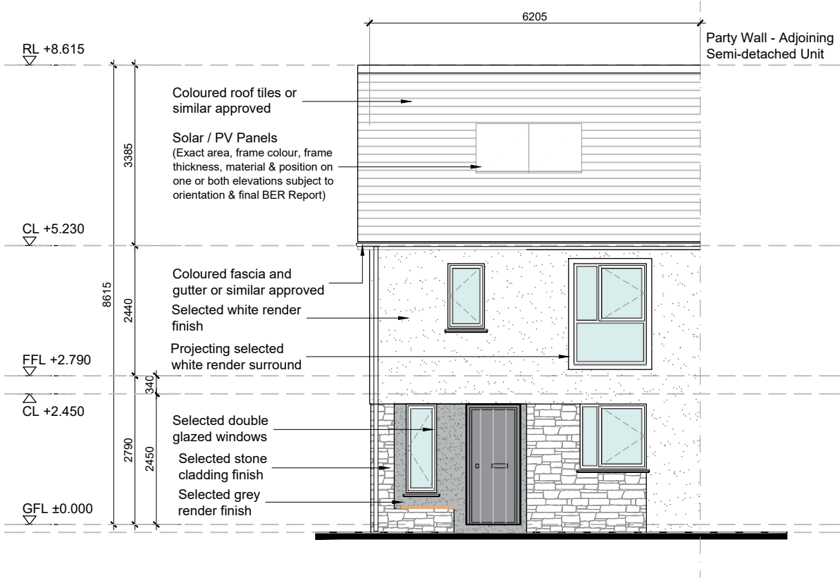
01 Front Elevation 1:100 @ A3
