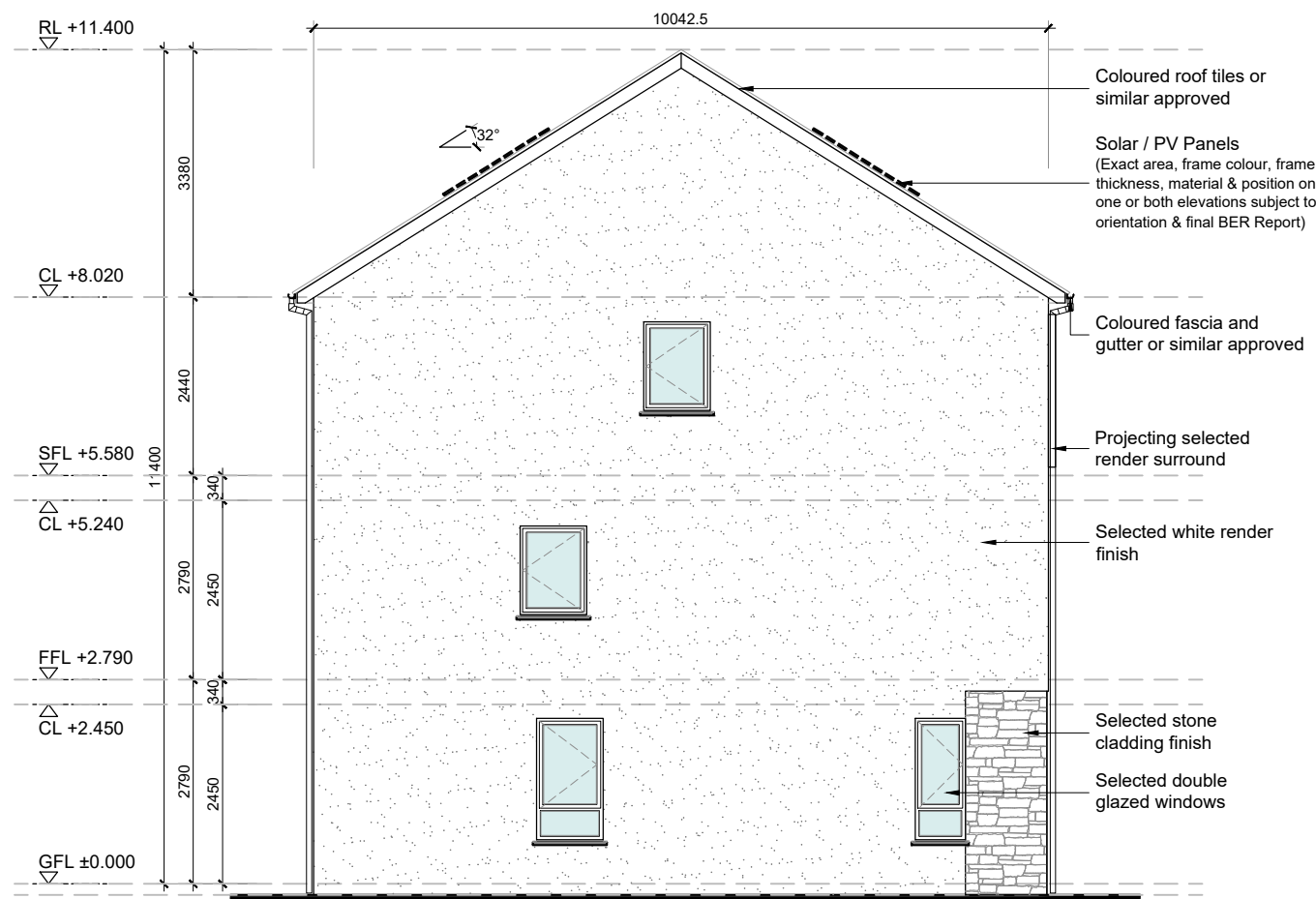
03 Side Elevation 1:100 @ A3
