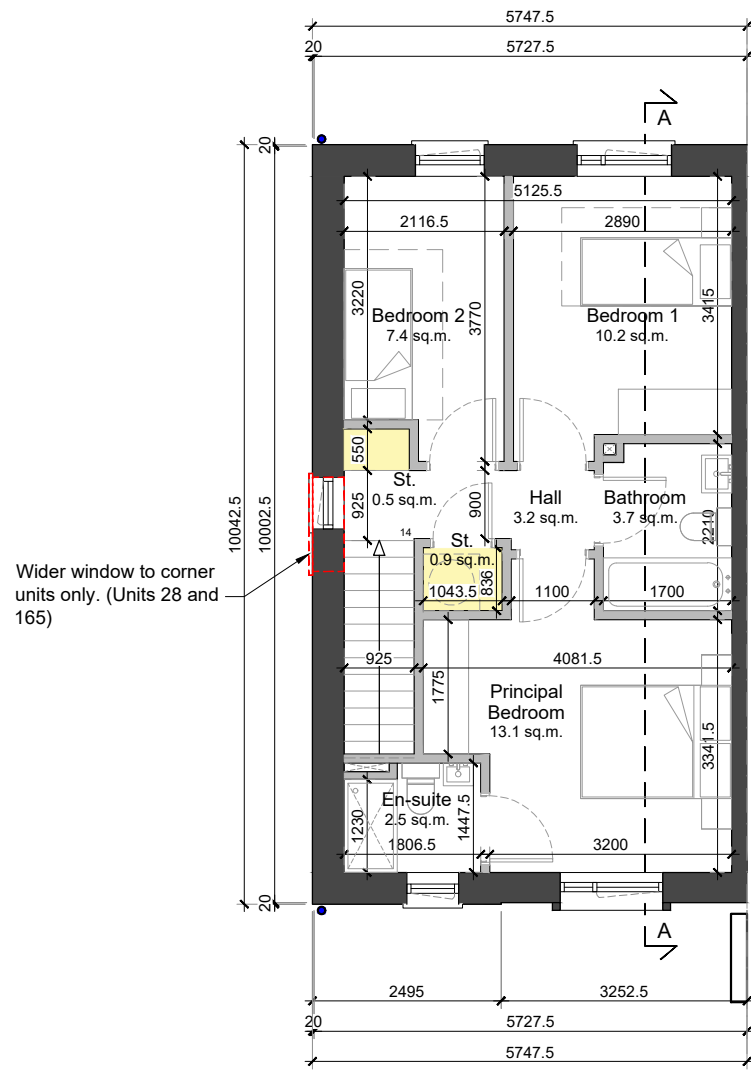
02 First Floor Plan 1:100 @ A3
