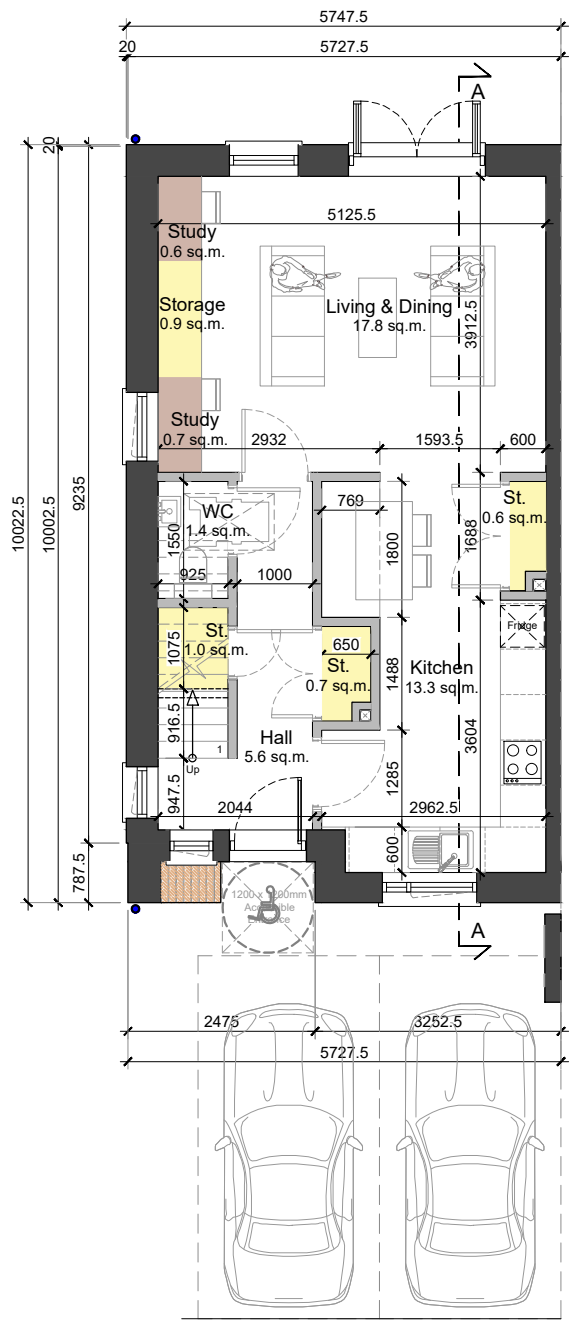
01 Ground Floor Plan 1:100 @ A3
